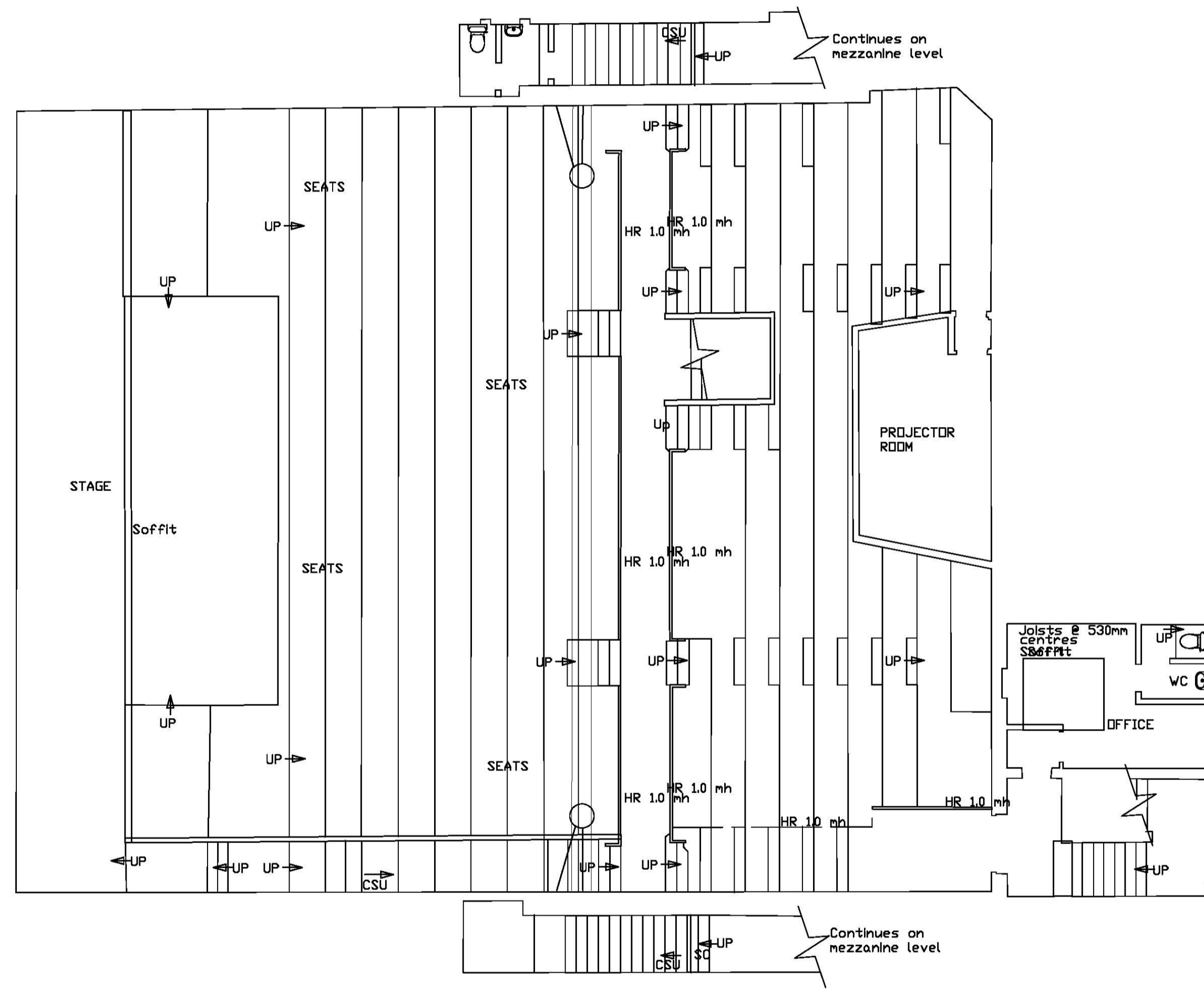
Existing First Floor Scale 1:100 @ A1
